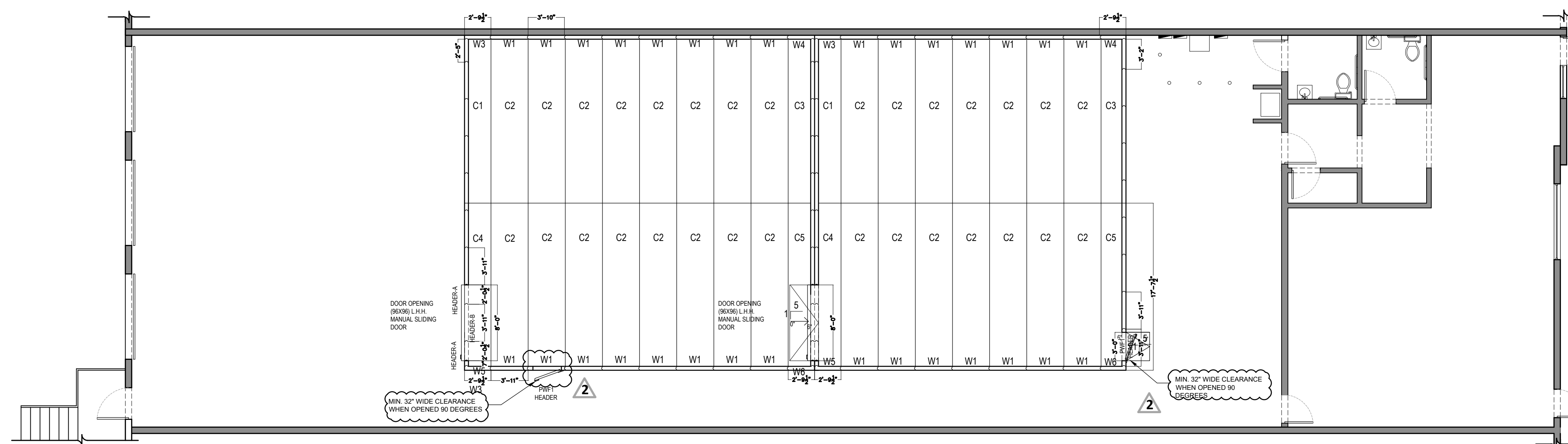
1 COOLER AND FREEZER PLAN A1.50 SCALE: 1/8
